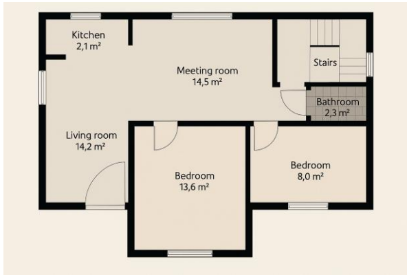
Fig. 1 Architectural layout of a single-story residential unit.
