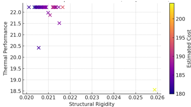
Fig. 6 Pareto Front Obtained Using a Genetic Algorithm for the Optimal Design of Construction Systems.
