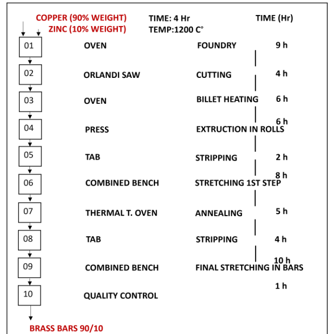
Fig. 8 Processing times for manufacturing the 90/10 brass bar
