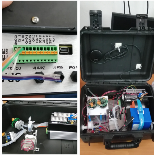
Fig. 4: Prototype of the proposed portable multi-sensor system.
