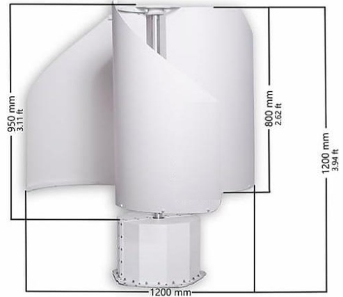
Fig. 2. Renova Wind EOS 1kW wind turbine. Source: https://renovawind.com/en/solutions/business-solutions
