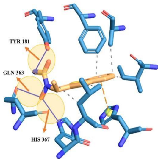
Fig 2: Interaction Protein-Zileuton
