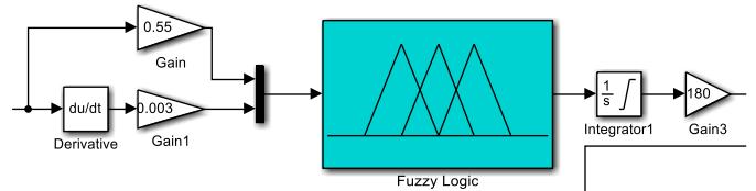
Fig. 7 FUZZY Control.
