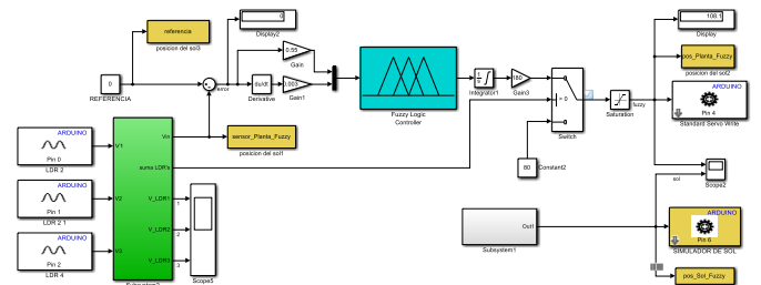
Fig. 8 FUZZY control algorithm applied to the prototype
