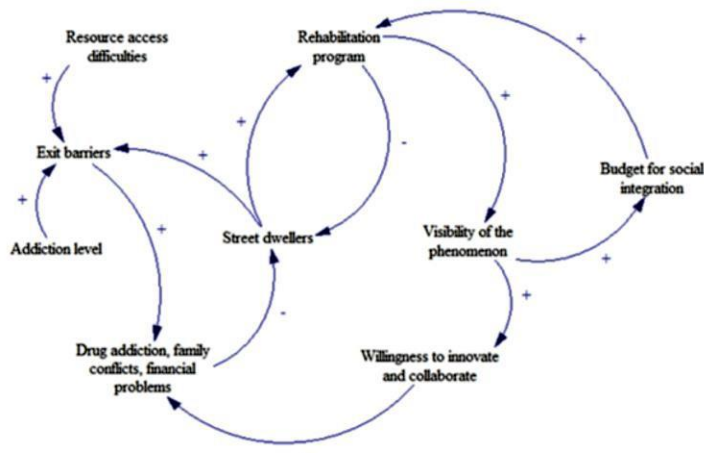
Fig. 3 Causal Diagram.
