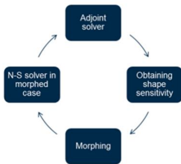
Figure 2: Adjoint optimization loop
