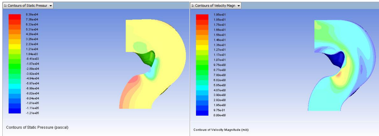
Figure 7: Pressure and velocity map for optimized model
