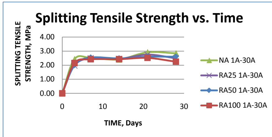
Figure 1: Results of Splitting Tensile Strength Testing For Concrete Mixes/Batches.
