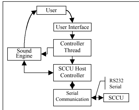
Figure 2. 3DSRE Components Diagram
